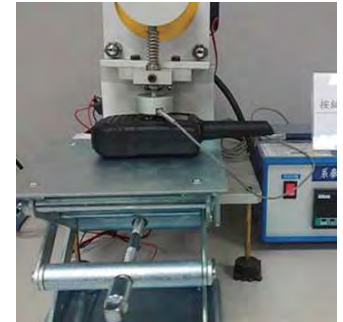
Key Switching Life Test
